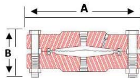
Threaded Offline
